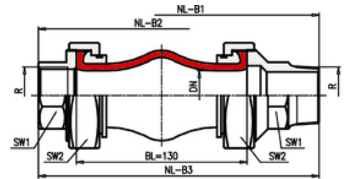
Note | Type B3 (internal-external thread) - Rubber Expansion Joint | dimensional sketch
