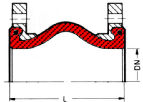
Note | Type A1 - Rubber Expansion Joint | dimensional sketch
