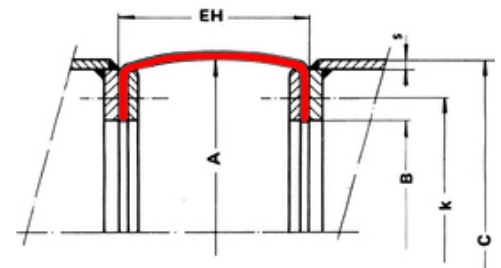
Note | Type 45 - Fabric Expansion Joint | dimensional sketch
