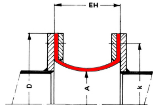
Note | Type 42 - Fabric Expansion Joint | dimensional sketch
